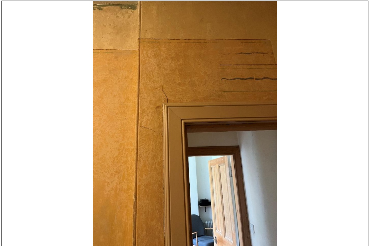
Figure 3 – Minor cracking around bedroom door frame.
