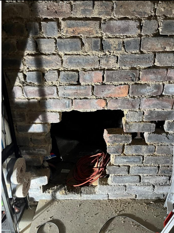
Figure 7 – Typical formed opening in underbuilding walls.
