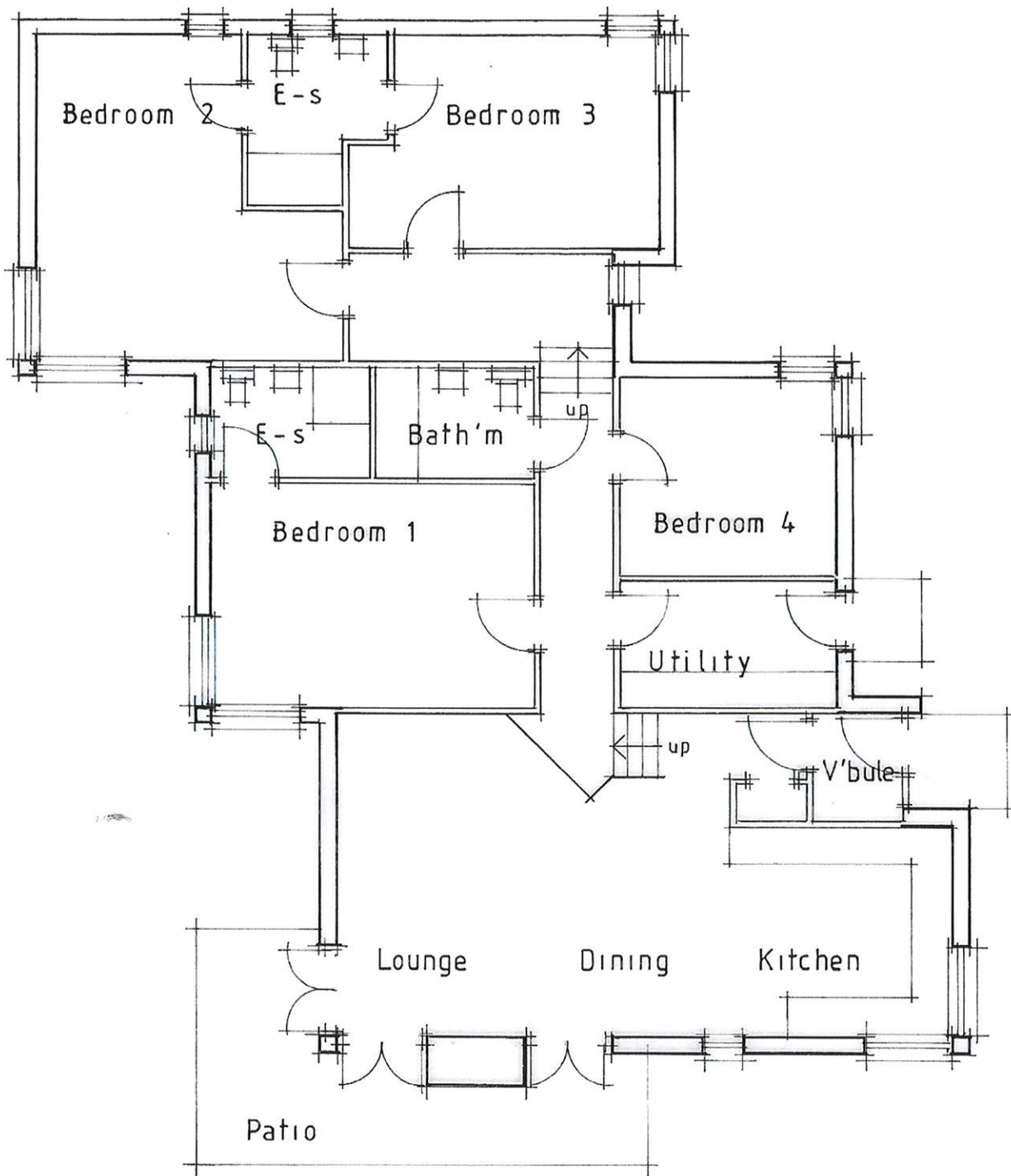
FLOOR PLAN
