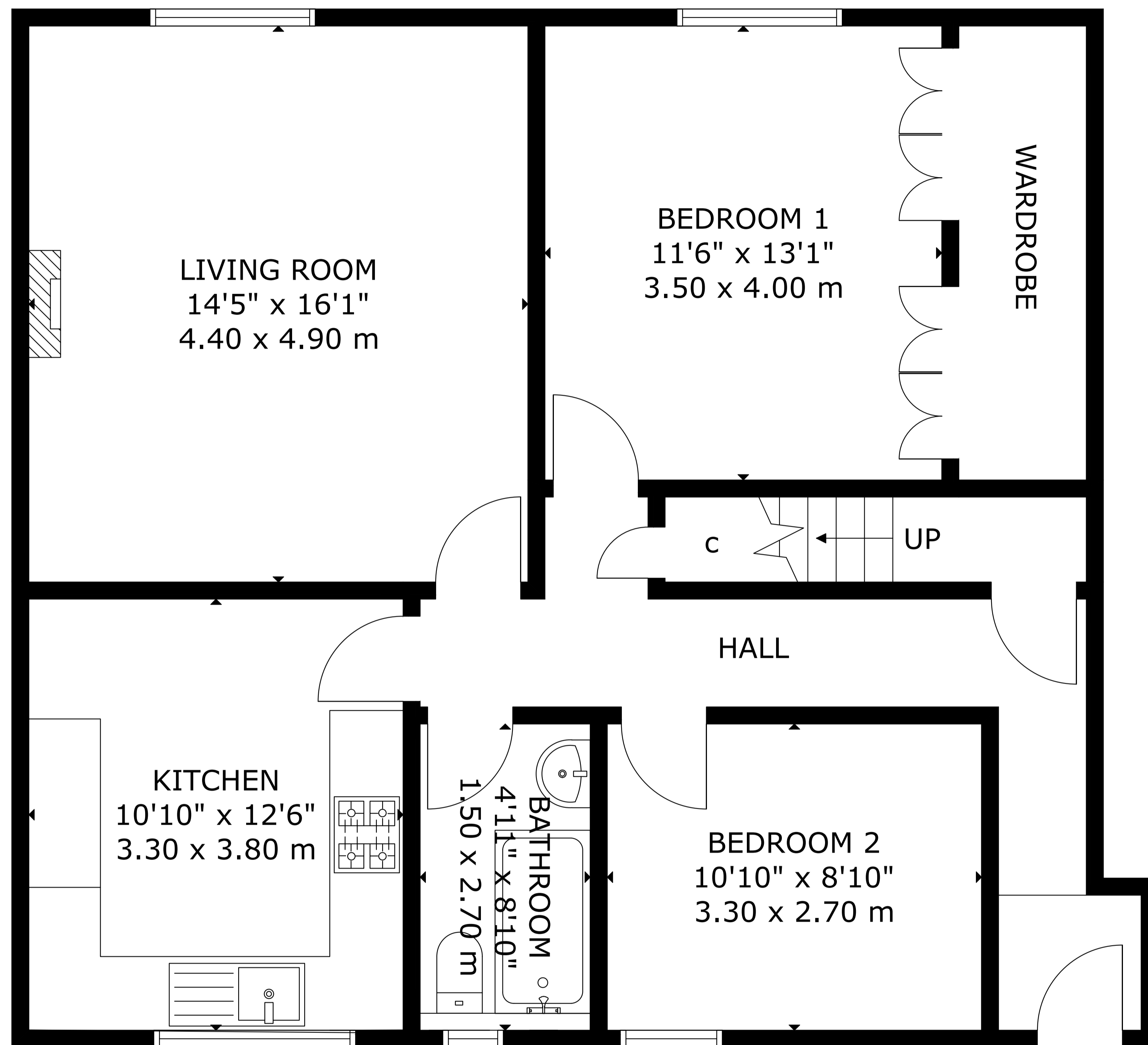
FIRST FLOOR
