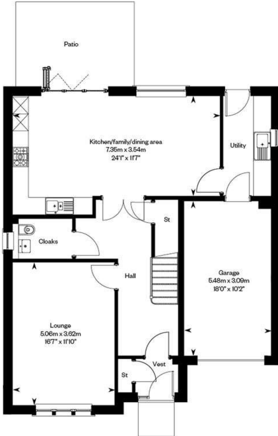
Ground floor
