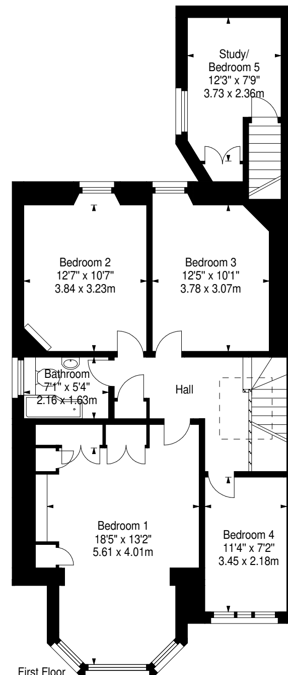
First Floor
