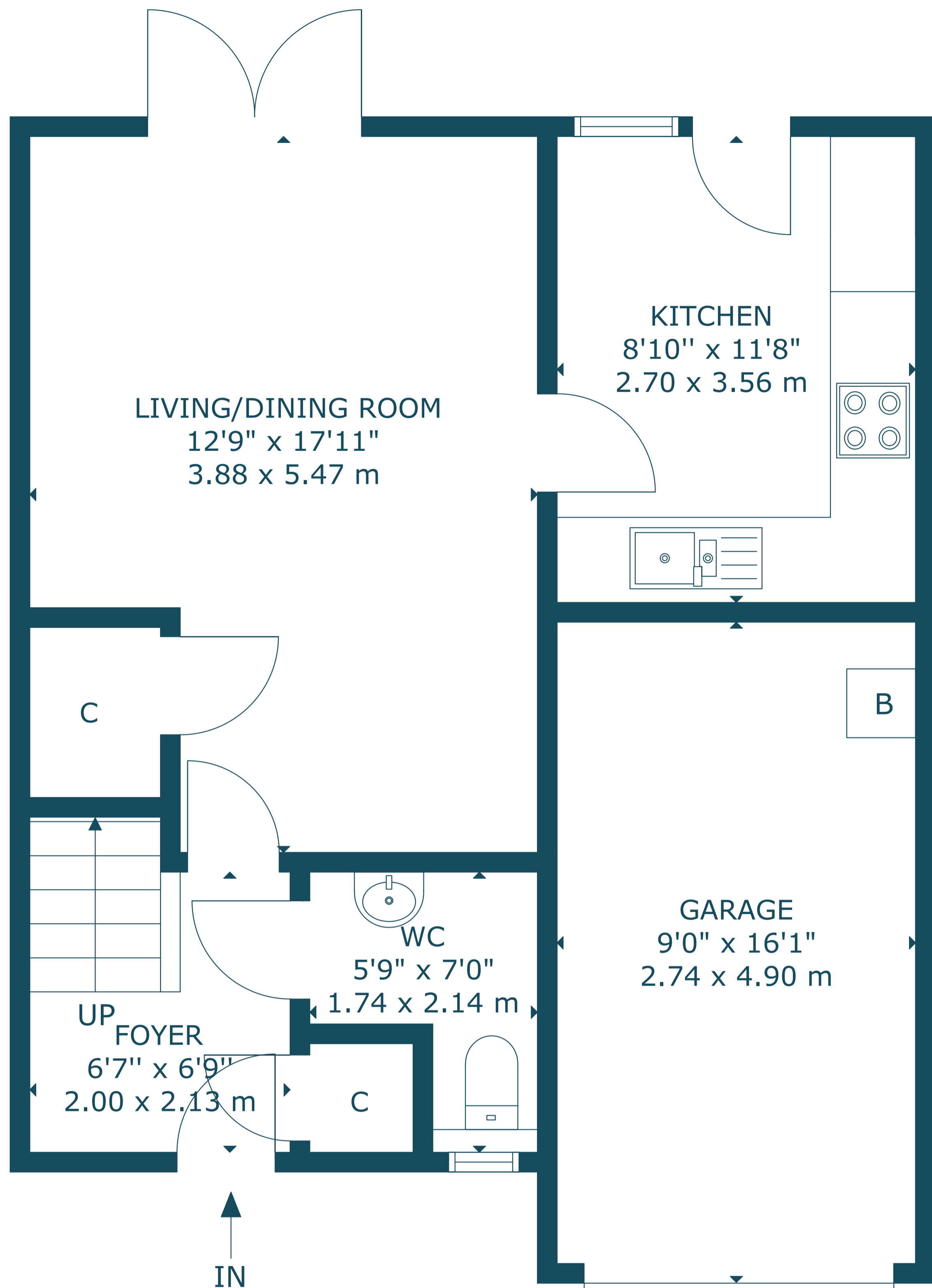
GROUND FLOOR
