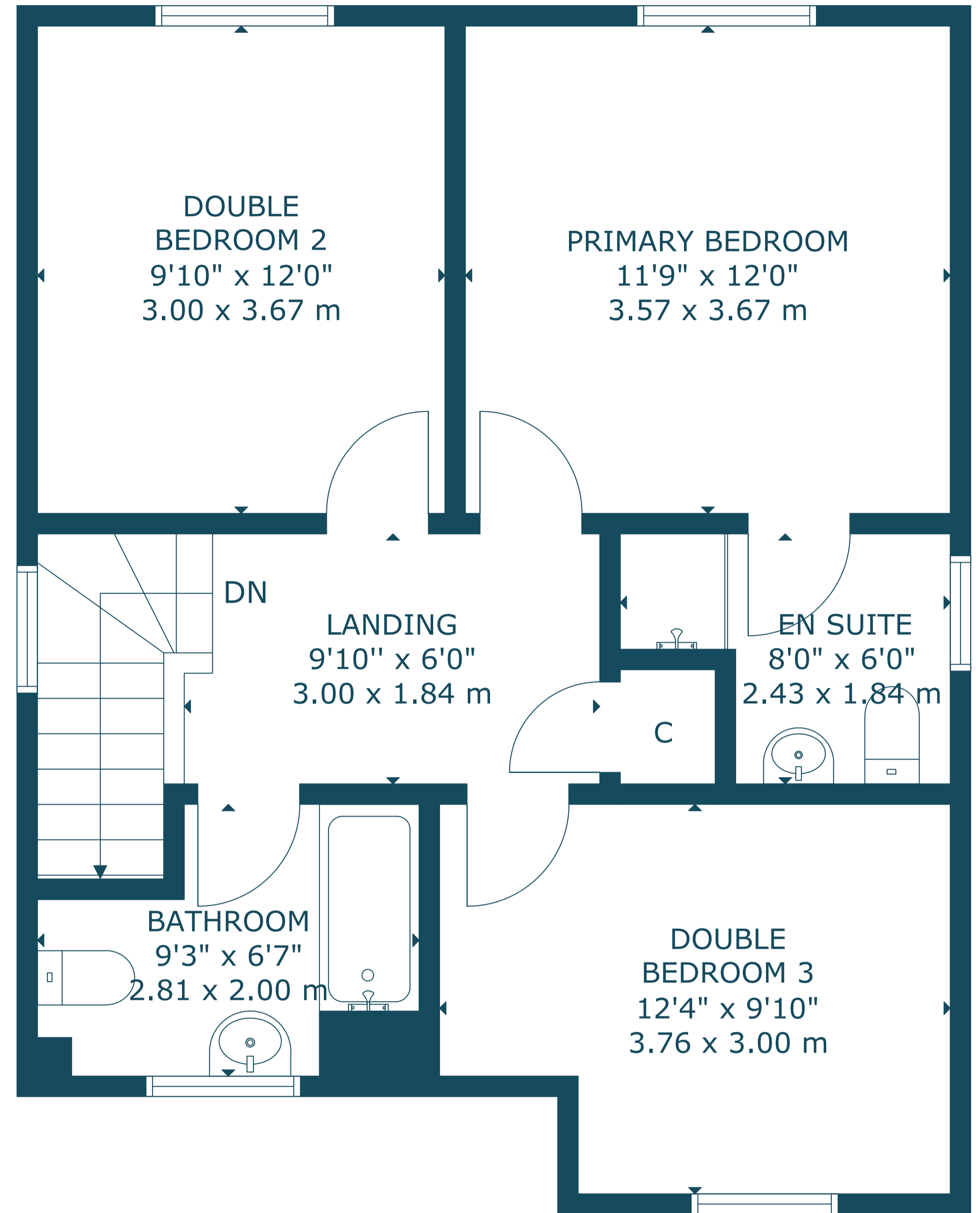
FIRST FLOOR
