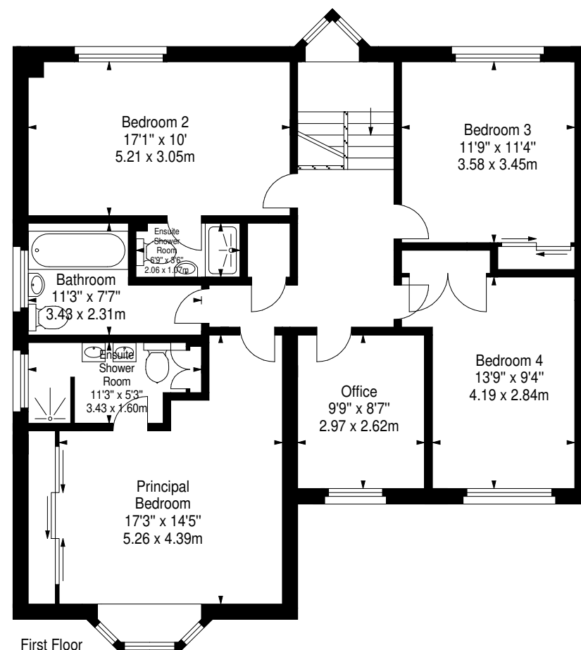
First Floor
