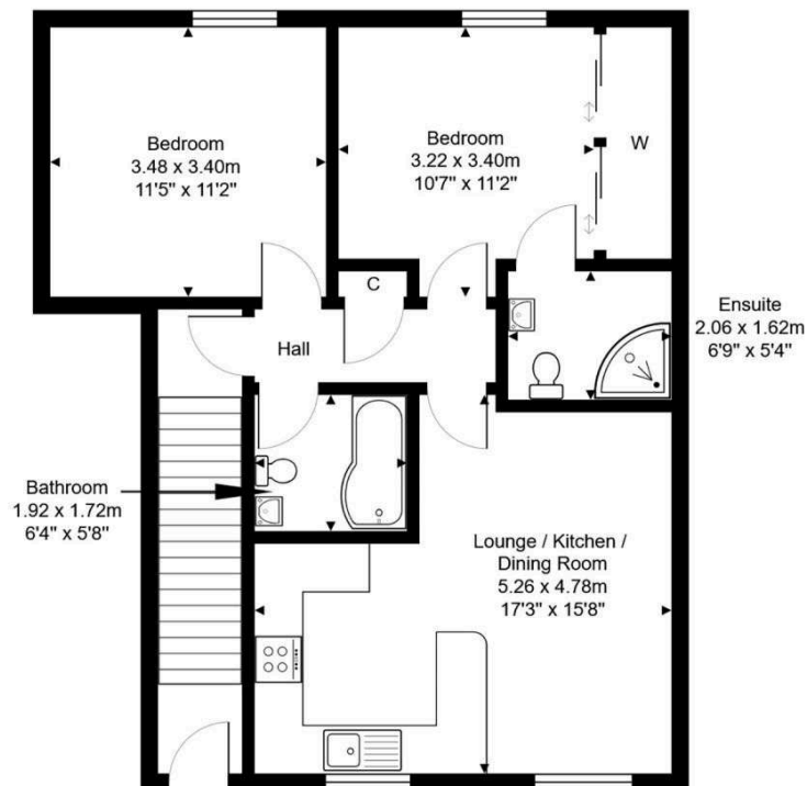
1st Floor
