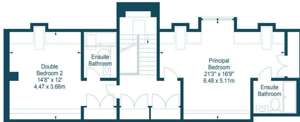
First Floor
